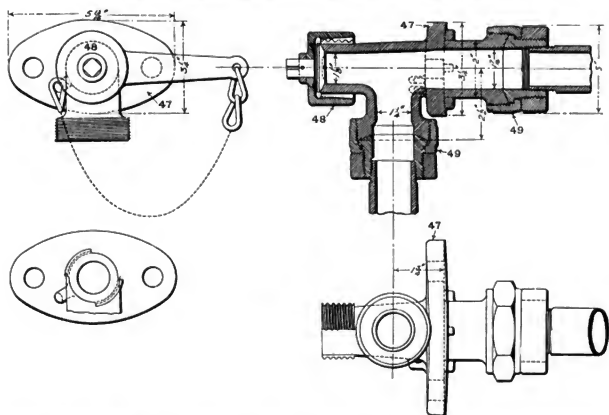
Figs. 390-393. 1½-in. Blower Pipe Connection. Atlantic (4-4-2) Locomotive. Pennsylvania Railroad.
